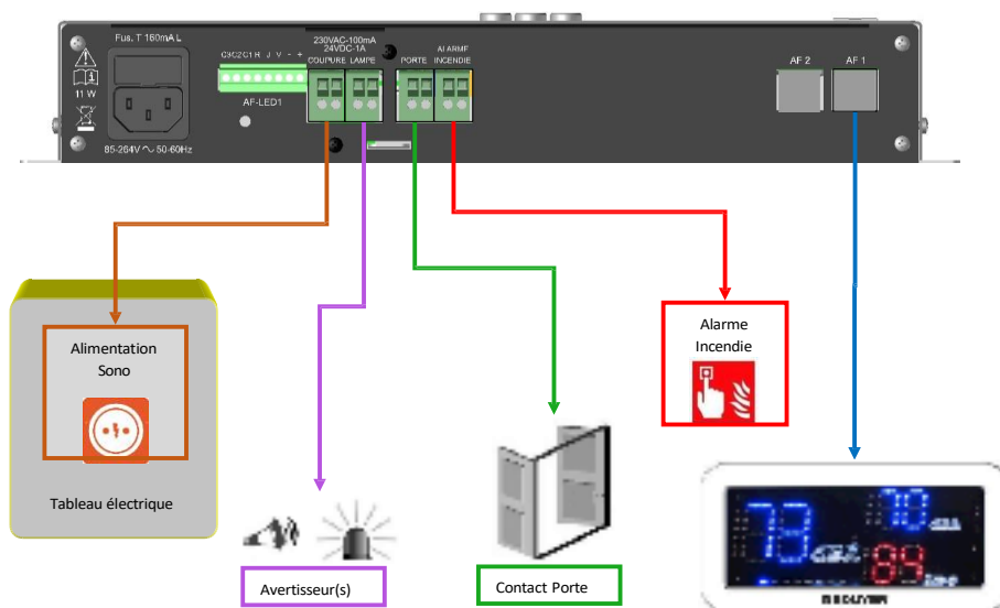
Figure 6. Raccordements sur le LC-1A
