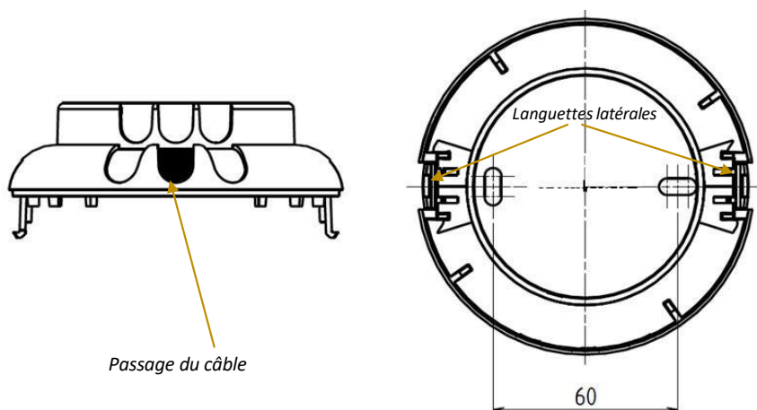
Figure 6. Fixation murale du GZ-CAPT 1
