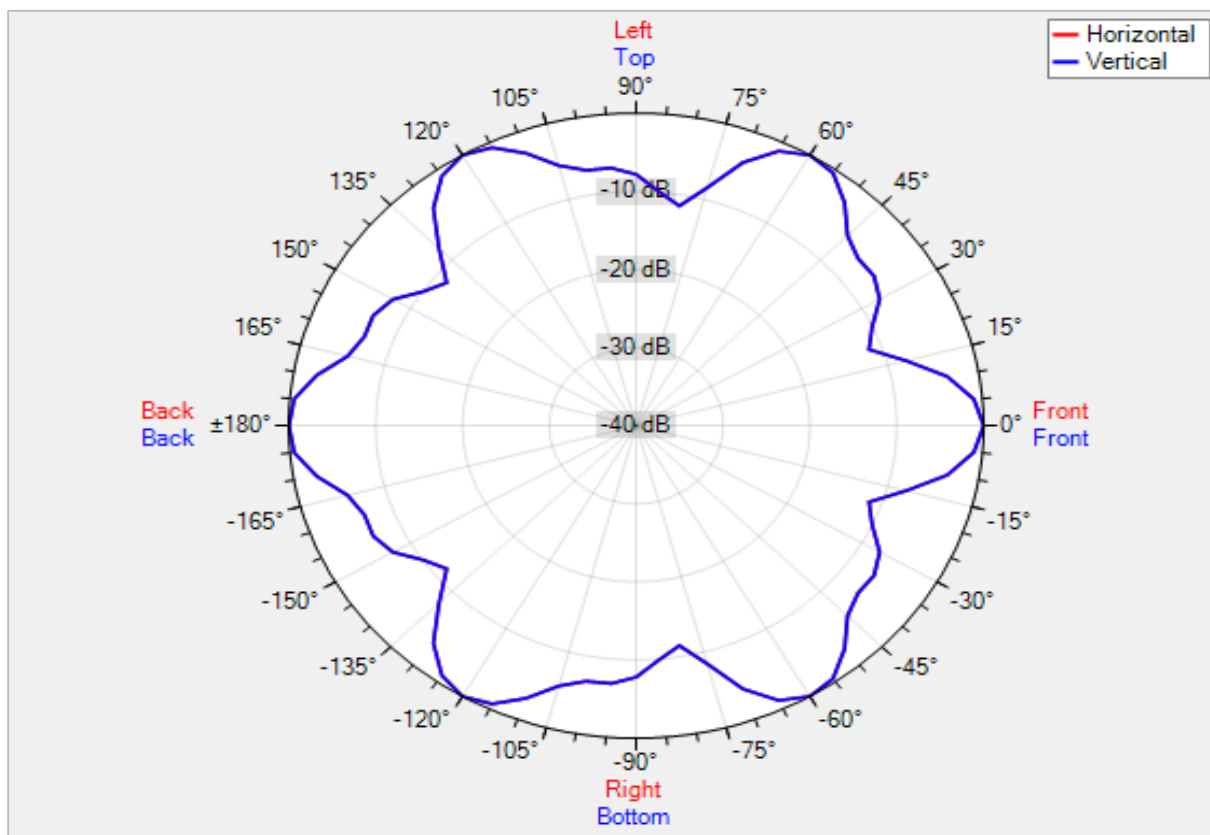
Directivity at 1 KHz
