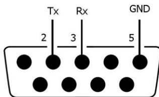
RS232 pinout
